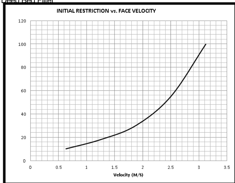
Deep Bed Filter
